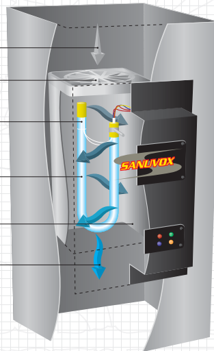
Ventilation Duct
