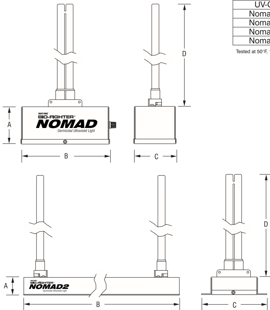
Fig. 1 Dimensions of single and dual bulb Triads.
